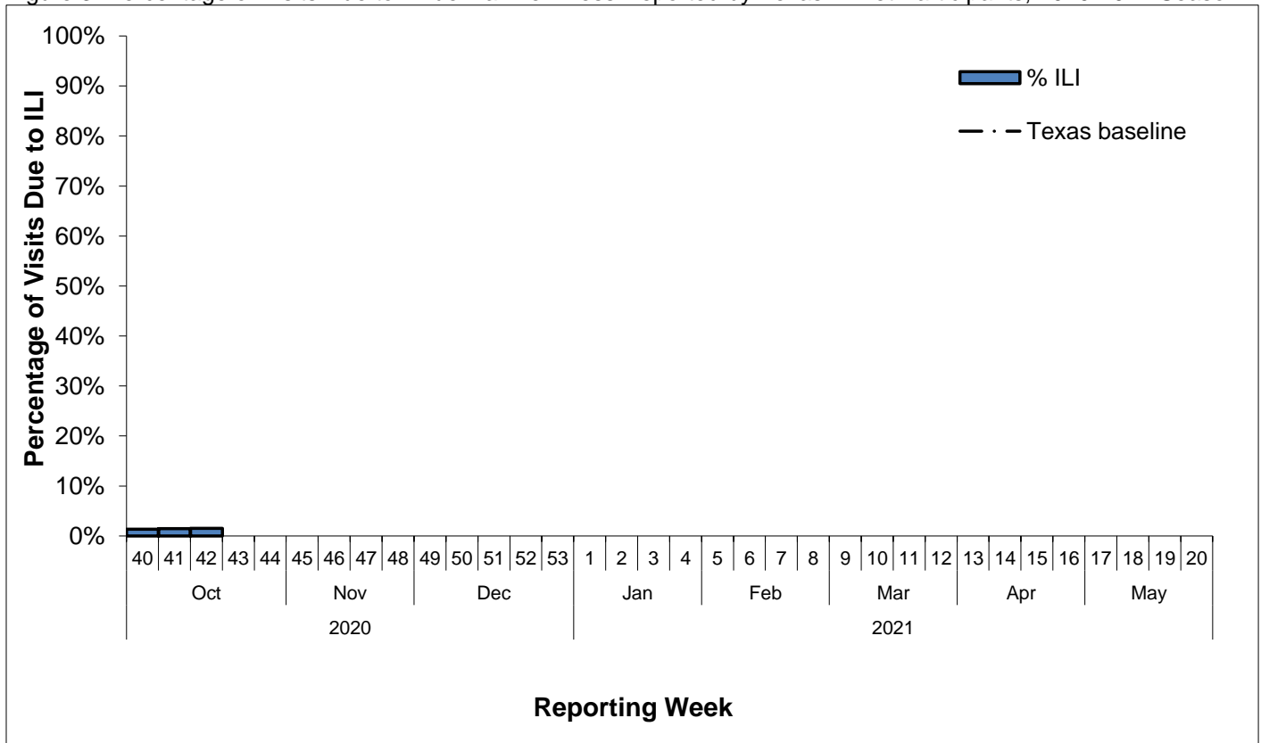
Figure 3: Percentage of Visits Due to Influenza-like Illness Reported by Texas ILINet Participants, 2020-2021 Season
