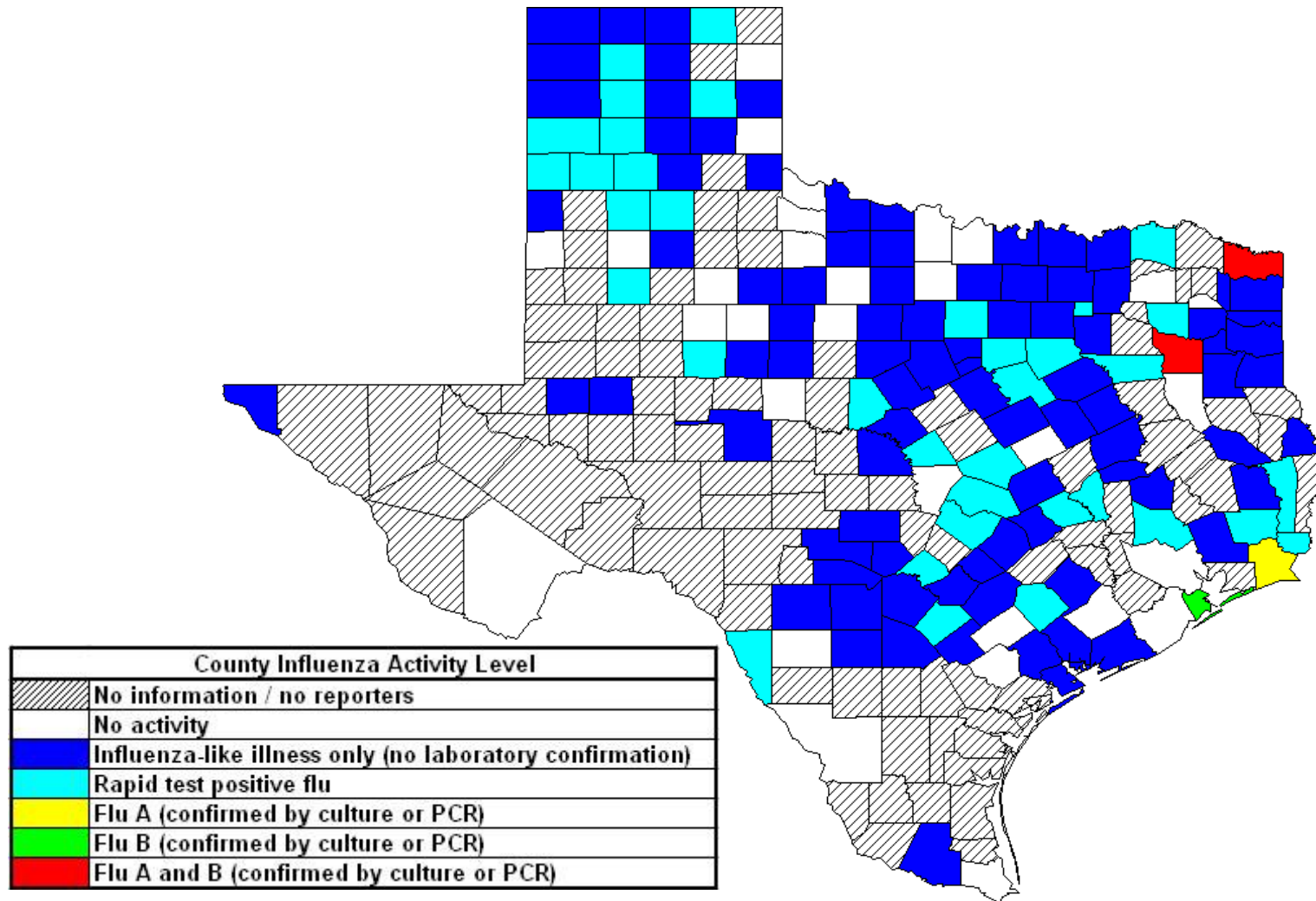
Figure 5: Texas Map Displaying the Highest Level of Influenza or ILI Activity Reported by County for the Week Ending Oct 17, 2020 (MMWR Week 42)
